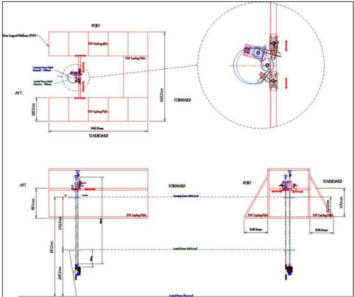
Figure 18 - Illustrating the proposed disposition of ROV Support Pole & the Pole Cam when simultaneously deployed into the Submarine
